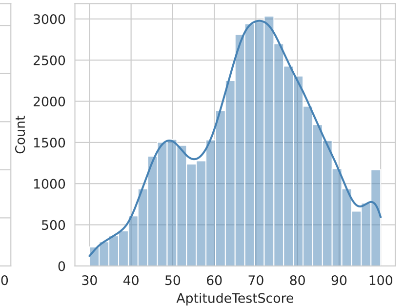
Distribution of AptitudeTestScore
